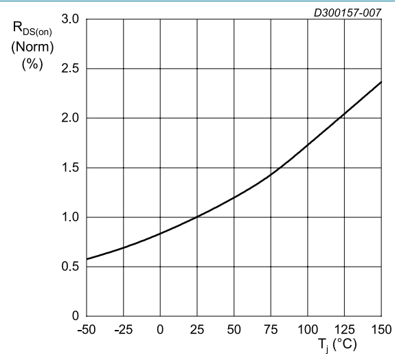
Fig. 7. Normalized drain-source on-state resistance as a function of junction temperature V_{GS} = 10\text{ V} ; I_D = 21\text{ A}
